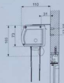
Lắp tường / Wall installation
