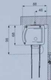
Lắp trần / Ceiling installation
